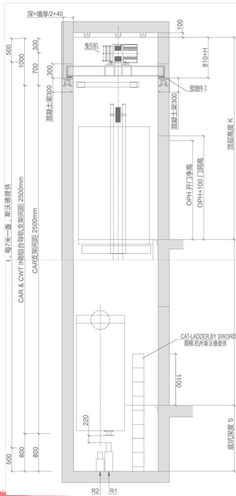
Elevation View
