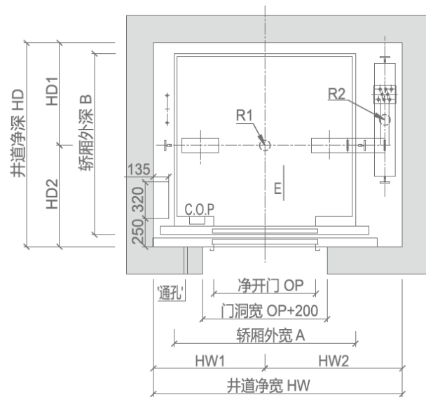
Hoist-way View
