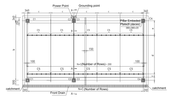
Architectural drawings
