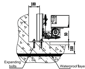
Component Diagram
